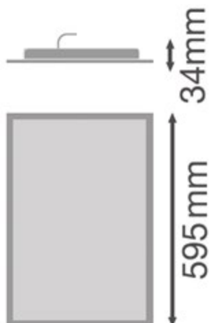
LED Panel 30*60
