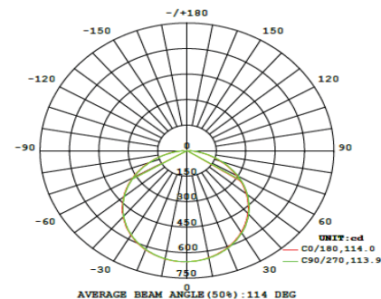
Light Distribution
