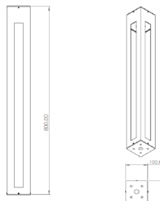
2D Dimensions
