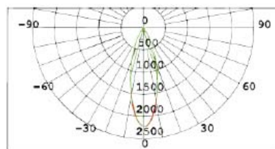
Light Distribution
