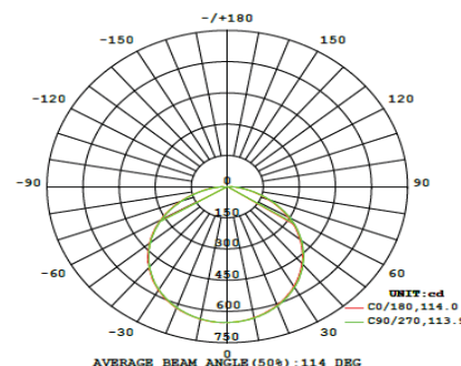
Light Distribution
